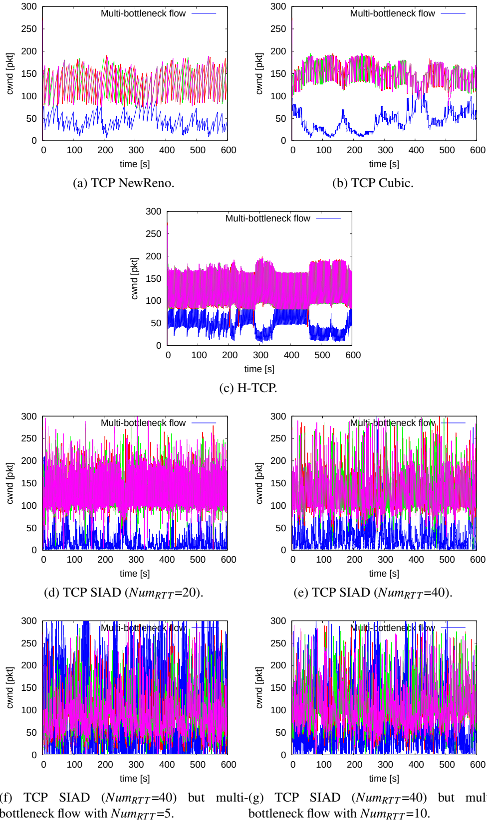
Figure C.6: Four TCP SIAD flows on 20 Mbit/s link and 0.5 \times \text{BDP} buffering with one flow crossing multiple bottlenecks.
