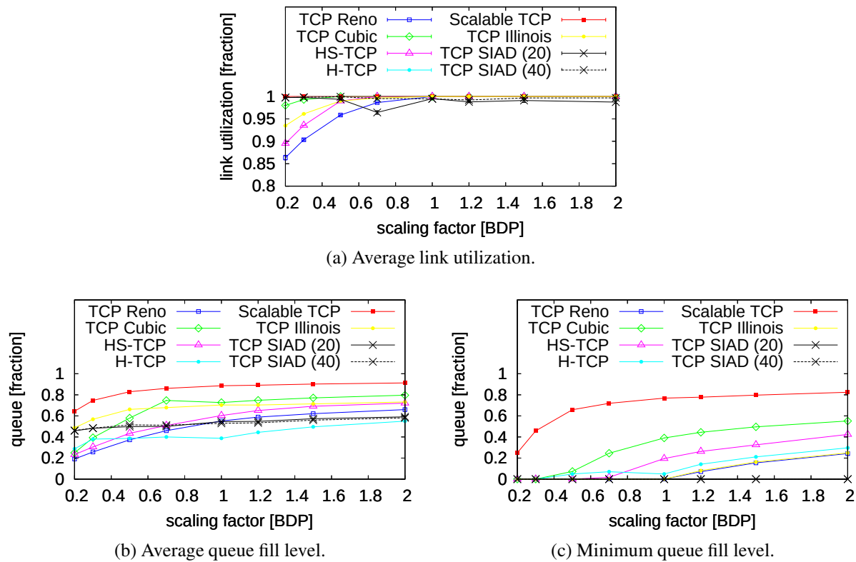
Figure 4.13: Single flow at 10 Mbit/s.
