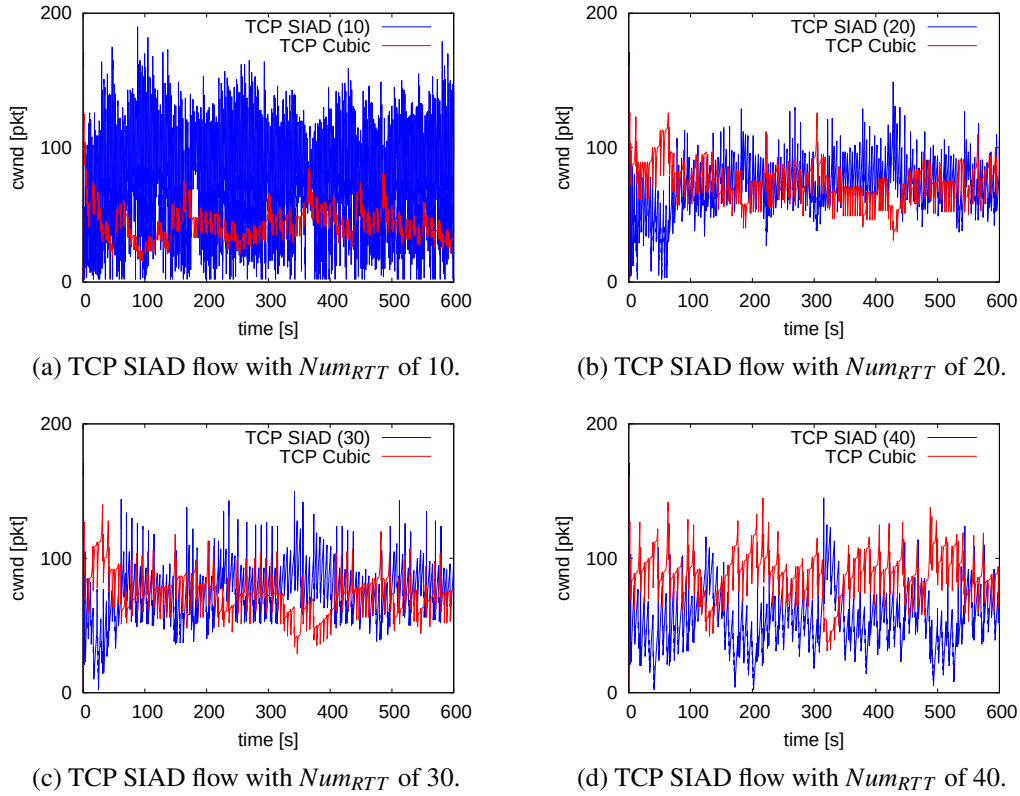
Figure 4.28: One TCP SIAD flow competing with one TCP Cubic flow on 10 Mbit/s link with 1 \cdot BDP of buffering.
