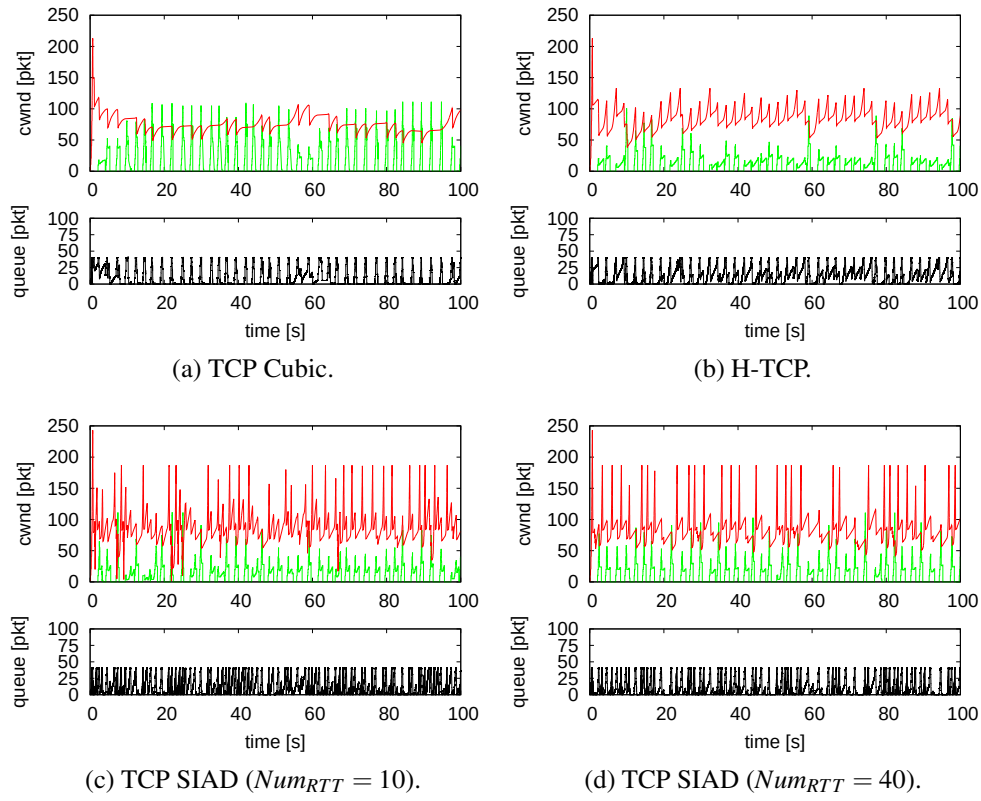
Figure C.16: One long-living flow with short flow cross traffic on 10 Mbit/s link and 0.5 \times \text{BDP} buffering.
