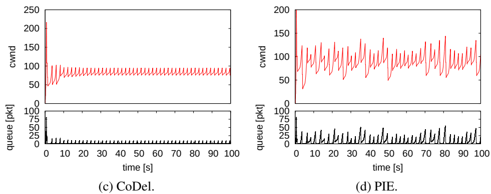
Figure C.19: H-TCP flow on 10 Mbit/s bottleneck link with different AQM schemes.
