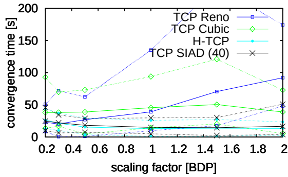
(a) 95% Average, min, and max convergence time ( Num_{RTT} = 40 ).
