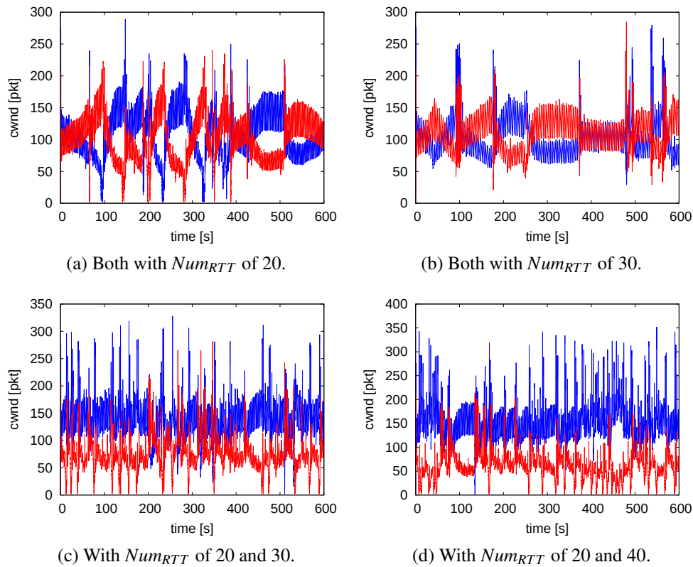
Figure 4.25: Two TCP SIAD flows on 20 Mbit/s link and with 0.5 \cdot BDP of buffering.
