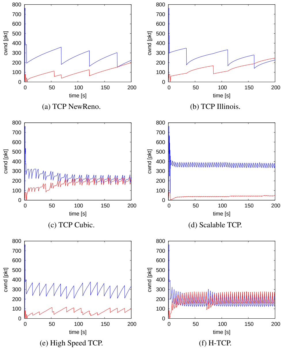
Figure C.7: Two flows on 20 Mbit/s link and 1.0 \times \text{BDP} buffering with different RTTs of 100 ms and 200 ms.
