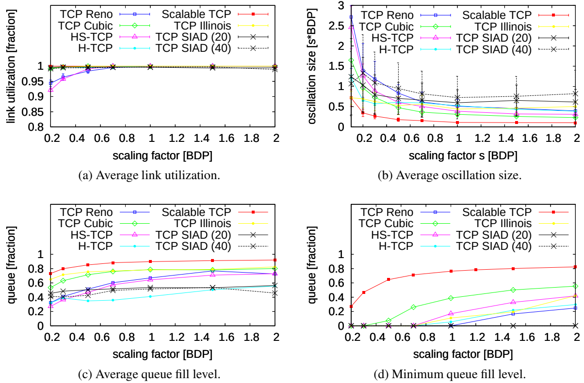
Figure 4.23: Two flows on 20 Mbit/s link.
