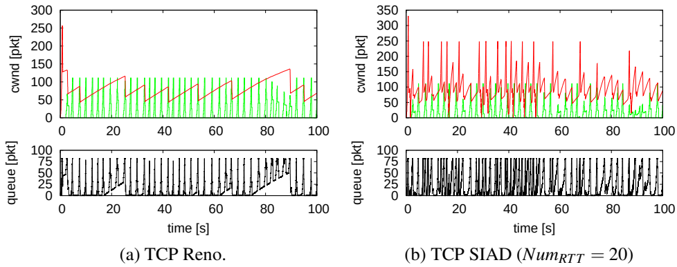
Figure C.15: One long-living flow with short flow cross traffic on 10 Mbit/s link and 1.0 \times BDP buffering.
