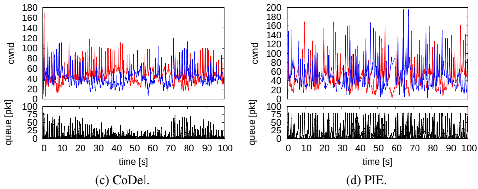
Figure C.20: Two TCP SIAD flows ( Num_{RTT} = 20 ) on 10 Mbit/s bottleneck link with different AQM schemes.
