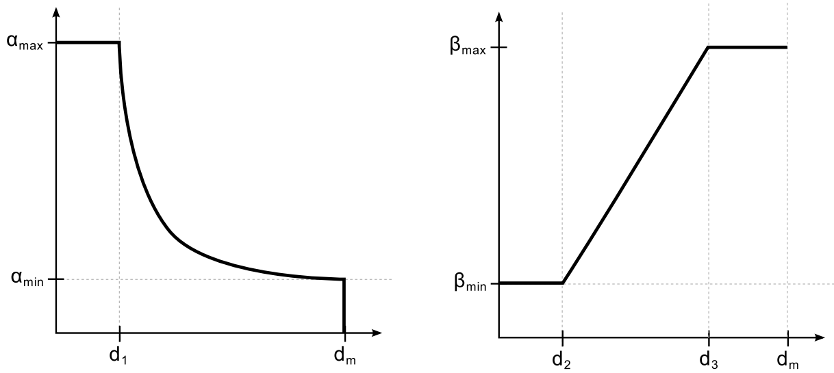
Figure 2.4: TCP Illinois: schematical curves for \alpha and \beta over d_a .
